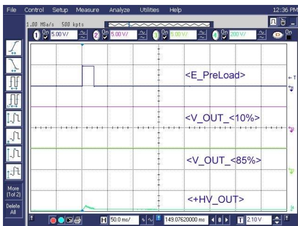
Figure 12: Switch-On Procedure Terminates During the First Preload Stage
