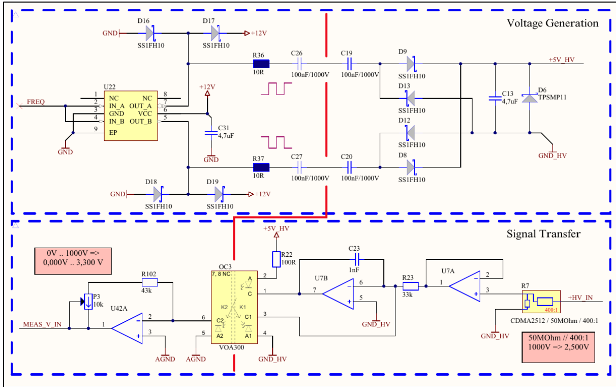
Figure 4: Connections between High Voltage and Control Side
