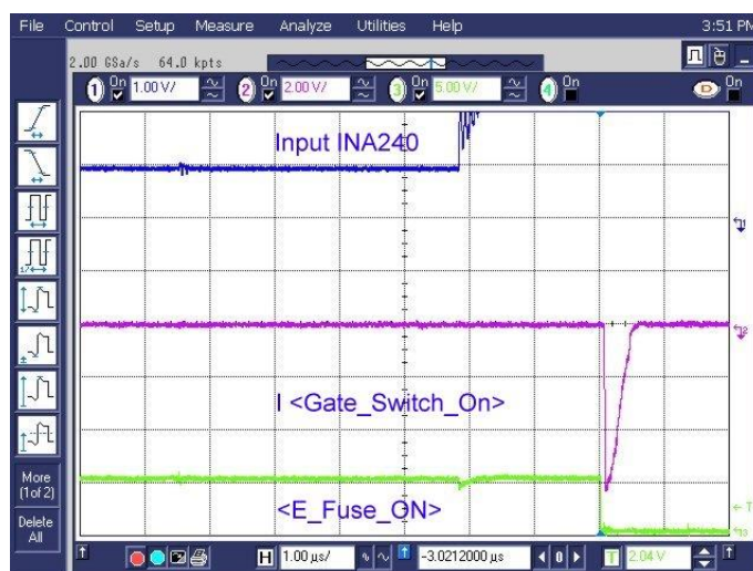
Figure 18: Switching Off after a Short Circuit Event
