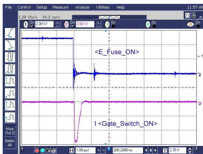
Figure 17: Switch-Off Procedure of the eFuse
