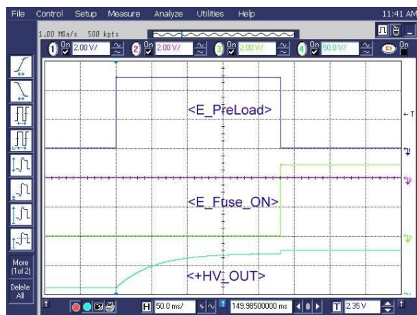
Figure 11: Successful Switch-On Procedure, First Preload Stage
