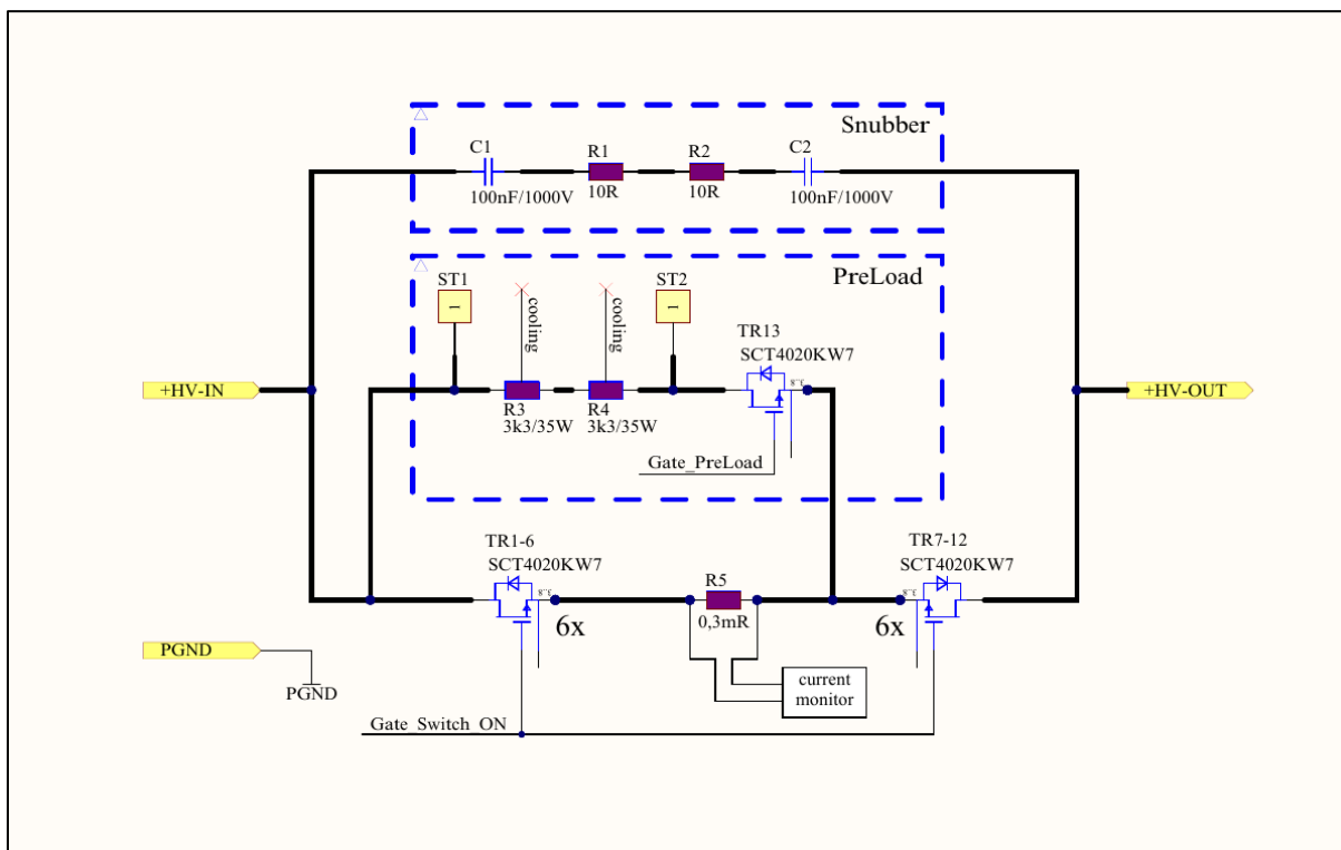
Figure 3: Overview of the High Voltage Side
