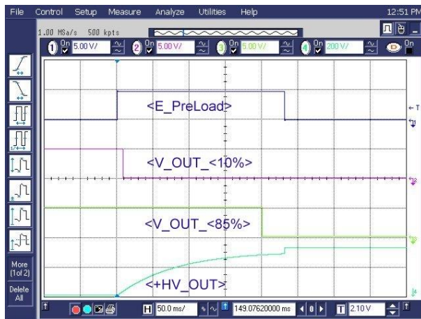
Figure 13: Successful Switch-On Procedure, Second Preload
