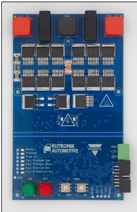
Figure 1: Vishay eFuse 800 VDC 50 A (Top View)
