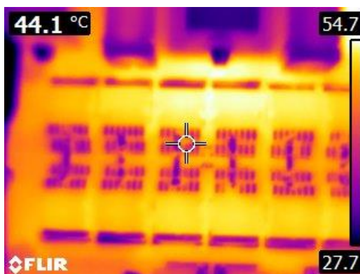
Figure 24: Stress Test with 40 A (20min)
