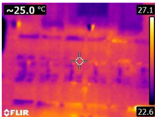
Figure 21: Stress Test with 10 A
