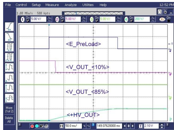
Figure 14: Switch-On Procedure Aborts During the Second Preload
