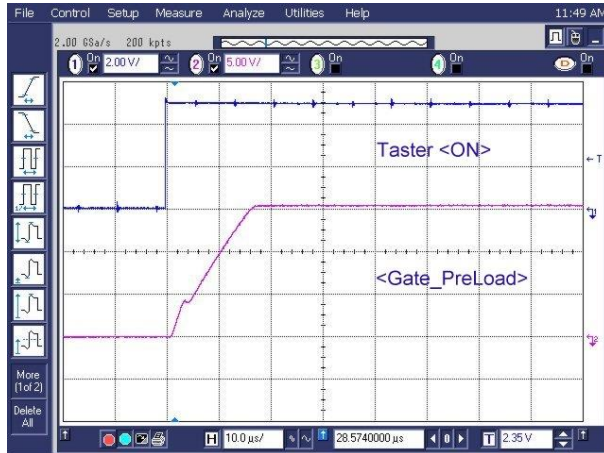
Figure 15: Switching on the Preload MOSFET
