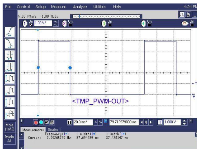
Figure 20: Temperature Measurement as seen at TP12
