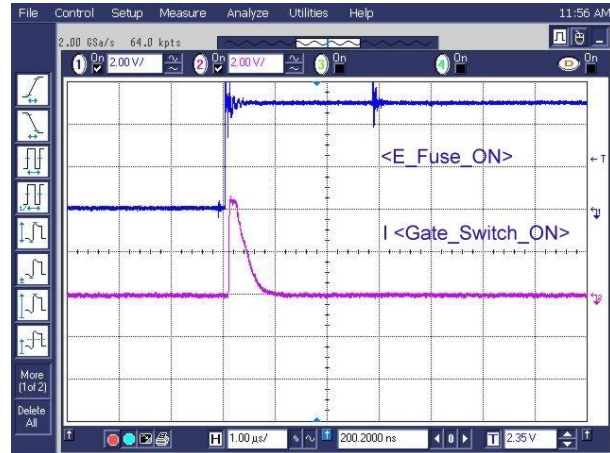
Figure 16: Switching on the Main MOSFETs
