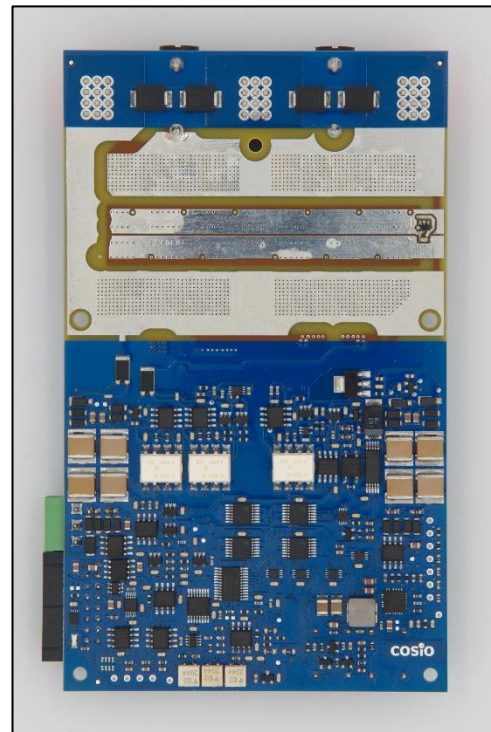
Figure 2: Vishay eFuse 800 VDC 50 A (Bottom View)
