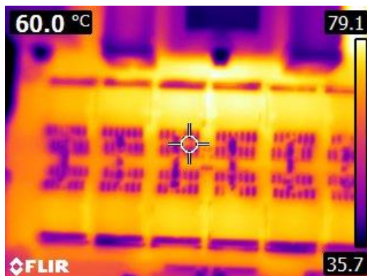
Figure 25: Stress Test with 50 A (60min)
