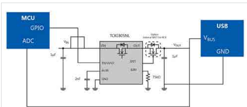
Figure 2: Protection of a USB charging socket using a TCKE805NL
