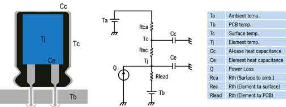
Figure 6: Thermal equivalent circuit diagram of the capacitors
