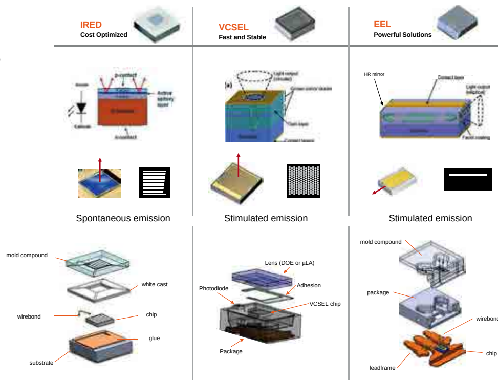
Comparison of chip technology and package for high-performance infrared LED, VCSEL, and edge-emitting laser (EEL)
