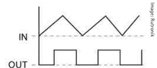
Figure 5: A Schmitt trigger converts slow edges into sharp rising edges.
