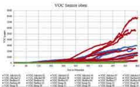
Figure 5: Concentration of VOCs as in Figure 4, but in the larger test space
