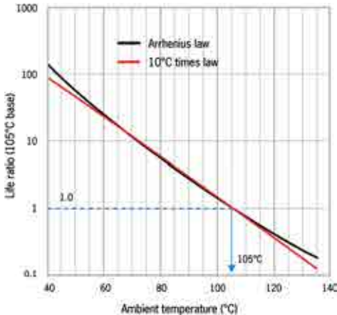
Figure 4: The Arrhenius equation and the rule of thumb that states the capacitor lifetime doubles with every 50 °F (10 °C) reduction in the operating temperature offer almost the same results.
