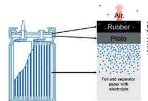
Figure 3: The electrolyte or liquid polymer diffuses during operation, resulting in a limited capacitor lifetime.
