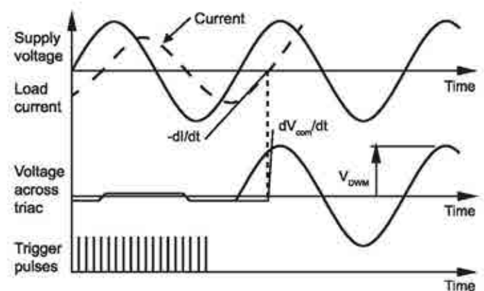
Figure 6: Commutation with inductive load
