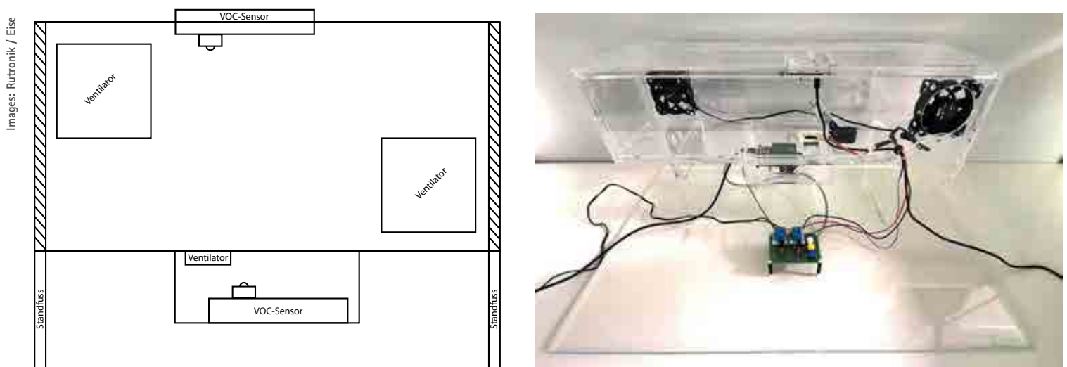
Figure 1: The measurement setup used to obtain reference data is very similar to the natural environment in which VOCs occur.
