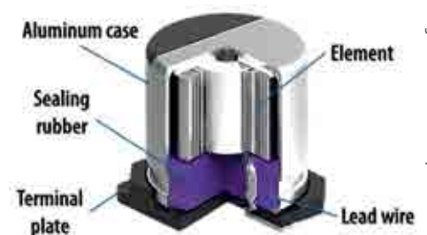
Figure 2: Basic design of electrolytic and polymer capacitors
