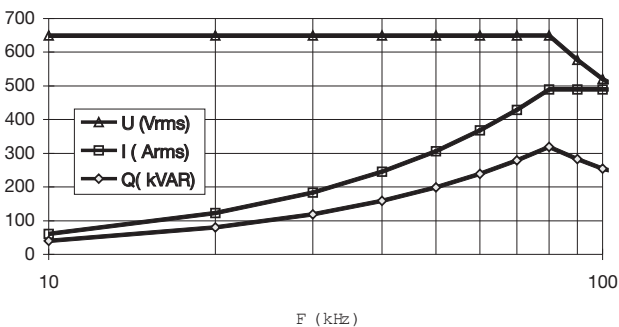
1.5 \mu F 650 Vrms Width 90 mm FAI66A0155K--
